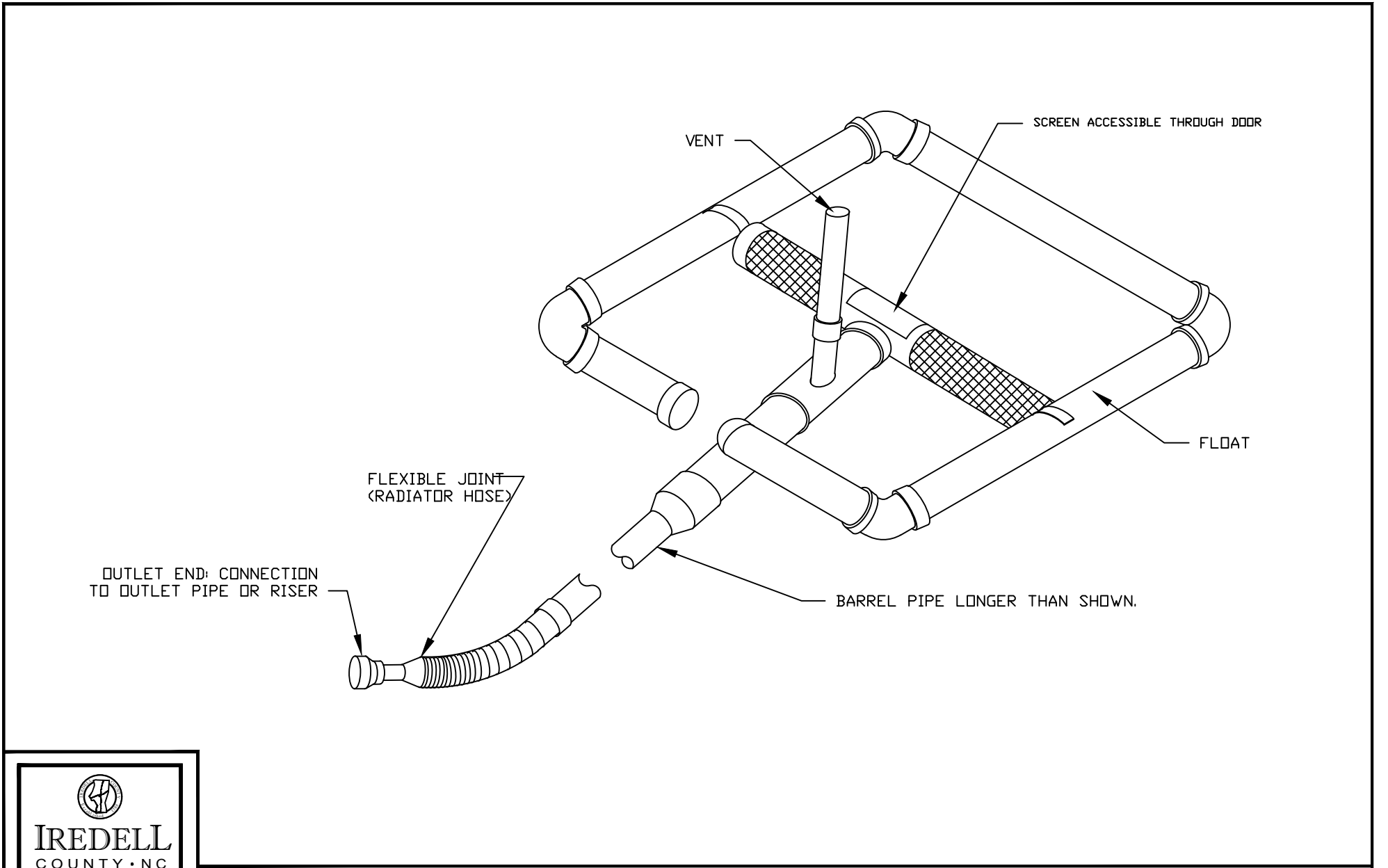
STANDARD SKIMMER DETAIL
