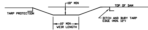
SECTION THRU WEIR
