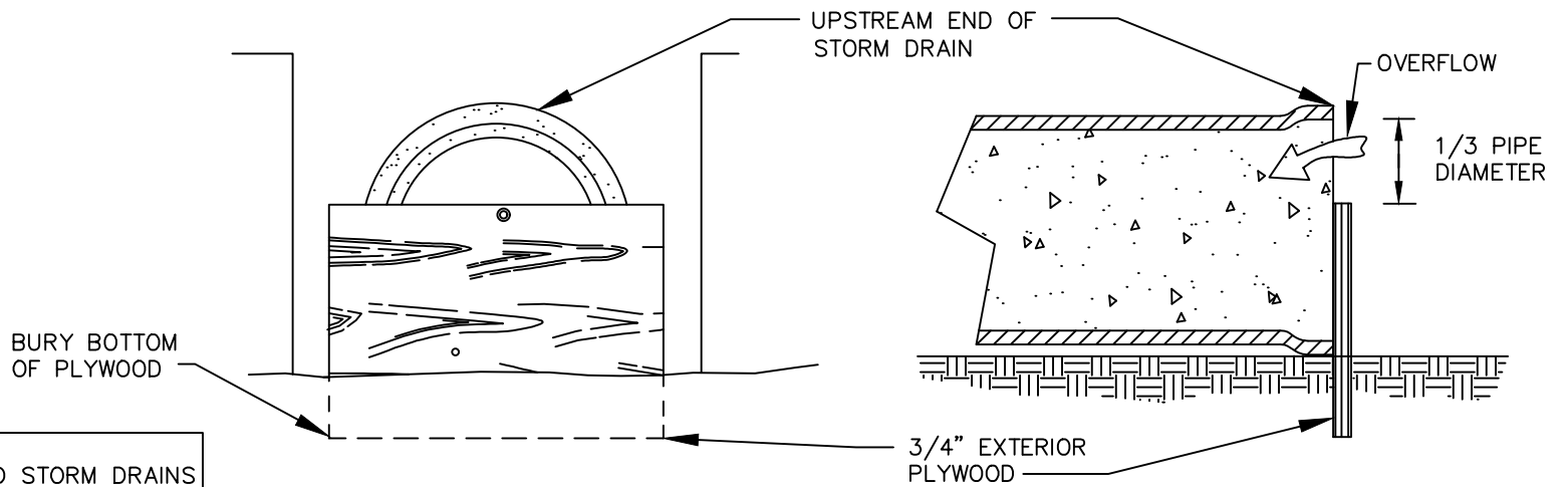
PLYWOOD INLET PROTECTION
